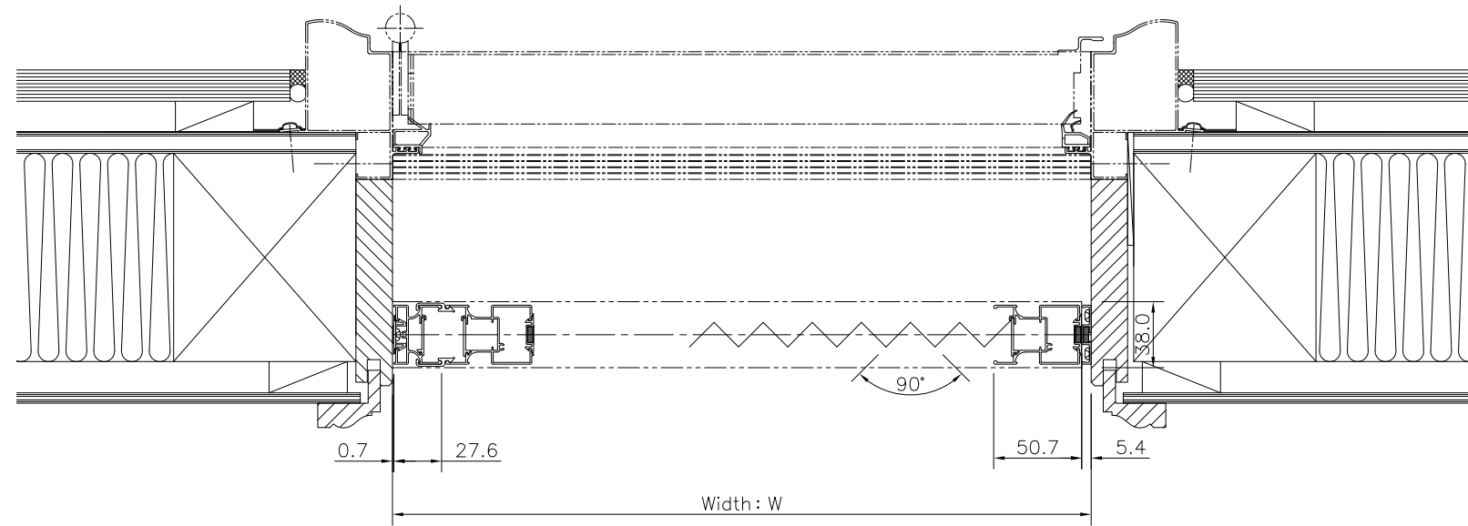
Zipooh Single door (8LME) Cross section
