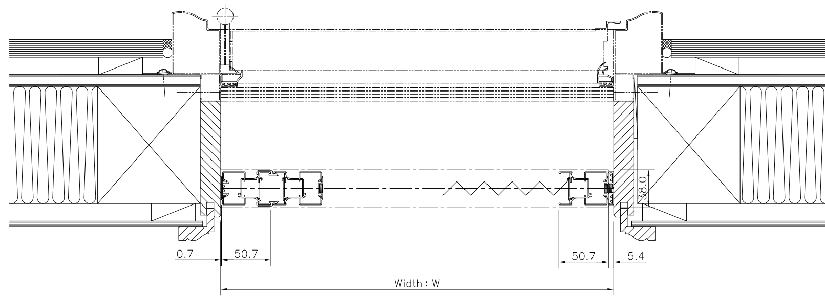
Zipooh Single door (88LME) Cross section
