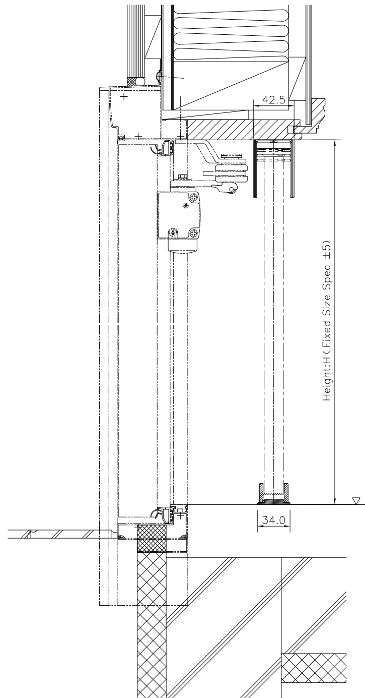
Shinpooh Longitudinal section
